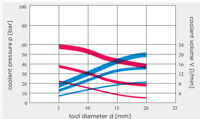
fig. 1: Required coolant pressures and volumes for RT 100 Ratio drills with internal spiral coolant ducts.
